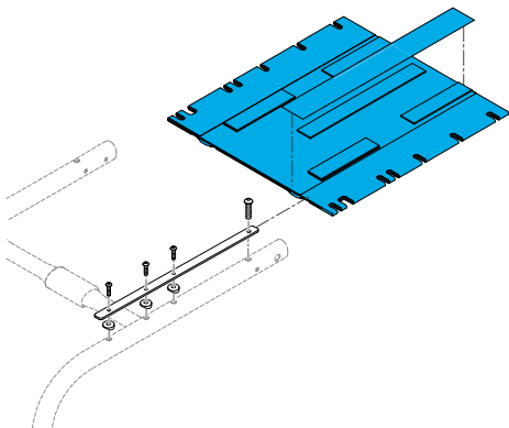
Quickie, Nitrum Seat Sling 12 " X __"; Order seat sling depth 1" shorter than back post depth
