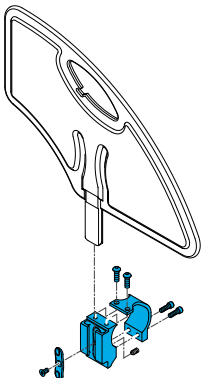
1579-115046 Quickie, Nitrum Plastic Side Guard Receiver Assembly Per Each
