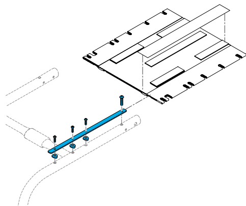
Quickie, Nitrum, Seat Rail Kit For __" Deep Chair
