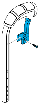
Quickie, Nitrum Backrest Upholstery Mounting Access Clip: For use with Push handles
