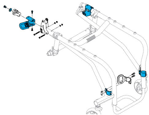
1579-168338 Quickie, Nitrum Hybrid Fixed Frame Transit Kit with Hardware
