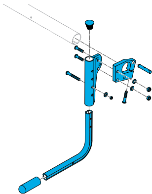
1579-164553 Quickie Rigid Chair, Tip Assist Complete Assembly
