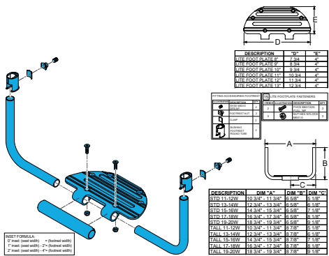
Quickie, Nitrum Ultra-Lite Aluminium Platform Footrest ____" Wide Long Assembly
