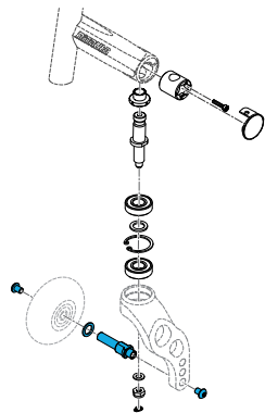
1579-159437 Quickie, Single Sided Fork Axle Set Per Side
