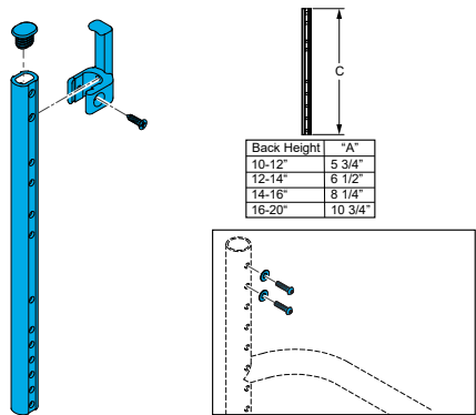
Quickie, Nitrum Height Adjustable Back Canes with Upholstery Mounting Clip, Without Push Handles, for Back Height ____ "
