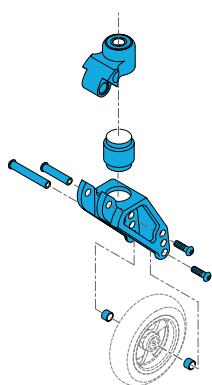
1579-50155 Quickie, Frog Leg Fork and Bearings; Without Elastomer
