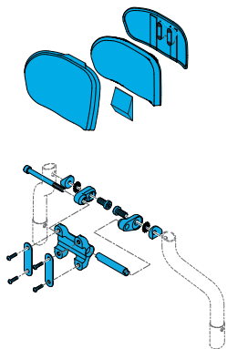
Quickie, Nitrum Freestyle Complete Aluminium Back-rest with Mounting Hardware __" x __" Tall
