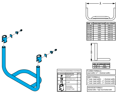
Quickie, Nitrum Standard Tubular Footrest, ____ " Wide with 75 Degree Footplate Angle
