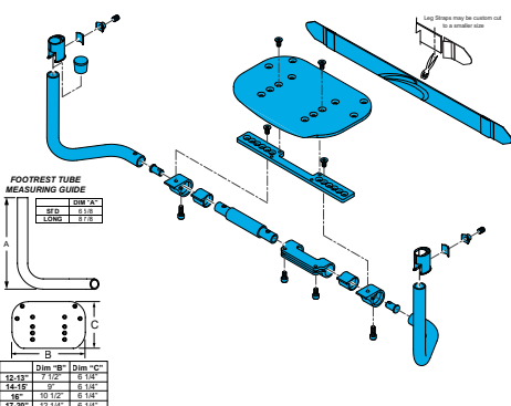
Quickie, Nitrum Composite Angle Adjustable Footrest Complete Short, ____" Wide Assembly
