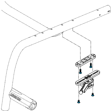
1579-164597 Quickie, Nitrum Center Direct Mount Compact Wheel Lock Hardware Kit
