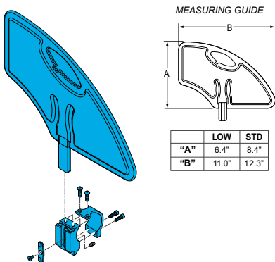
1579-115048 Quickie, Nitrum Small Plastic Side Guard Assembly Pair with Receivers
