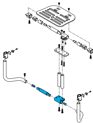
Quickie, Nitrum Adaptive Footrest Centre Mounting Kit 8 & 10" Wide
