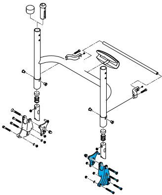
Quickie, Nitrum Ultra Light Weight Back Frame Bracket/Seat Lail Mount Left Side Only
