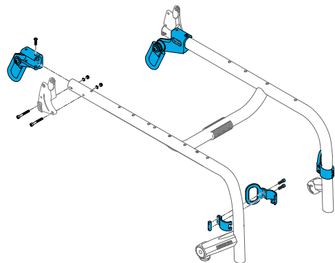
1579-164348 Quickie, Nitrum Standard Depth Adjustable Frame Transit Kit with Hardware
