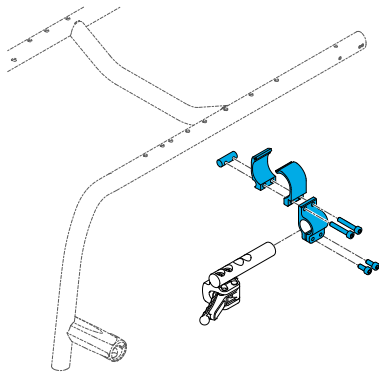
1579-76805005 Quickie, Wheel Lock Oval Frame Clamp, Universal
