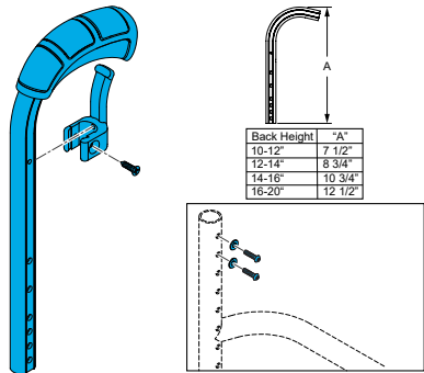
Quickie, Nitrum Height Adjustable Push Handle with Upholstery Mounting Clip for ____ " Back Height
