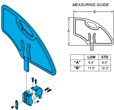
1579-115047 Quickie, Nitrum Standard Plastic Side Guard Assembly Pair with Receivers
