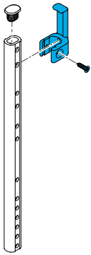
Quickie, Nitrum Backrest Upholstery Mounting Access Clip: For use without Push handles
