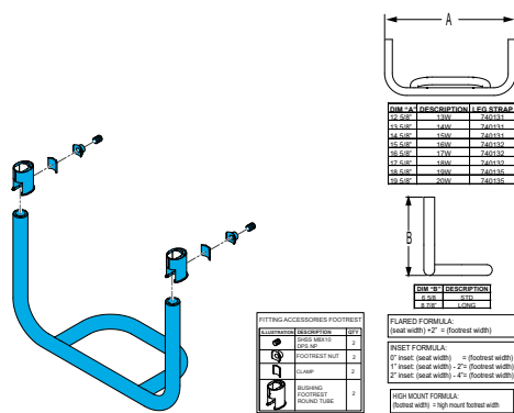
Quickie, Nitrum Long Tubular Footrest, ____ " Wide with 75 De- gree Footplate Angle
