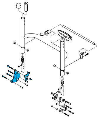
Quickie, Nitrum Ultra Light Weight Back Frame Bracket/Seat Rail Mount Right Side Only
