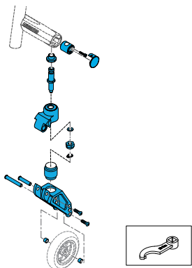
Quickie Nitrum, Frog Leg Suspension, ___ Fork and Stem Assembly
