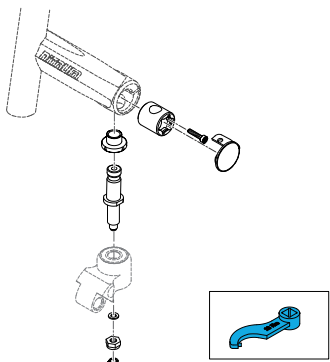
1579-116351 Quickie, Frog Leg Fork Assembly Tool
