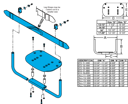
Quickie, Nitrum Composite Footrest Complete Short ____" Wide Assembly
