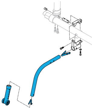
Quickie Rigid Chair, Anti-tip Regular Assembly ____ Side for ____ Rear Wheels
