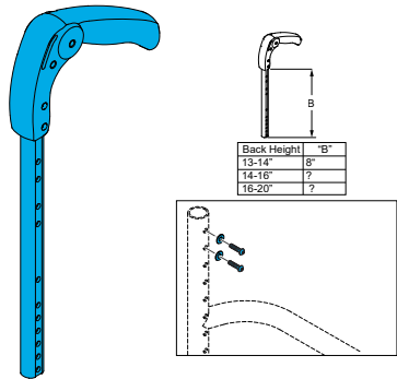
Quickie, Nitrum Height Adjustable Folding Push Handle with Upholstery Mounting Clip for ____ " Back Height
