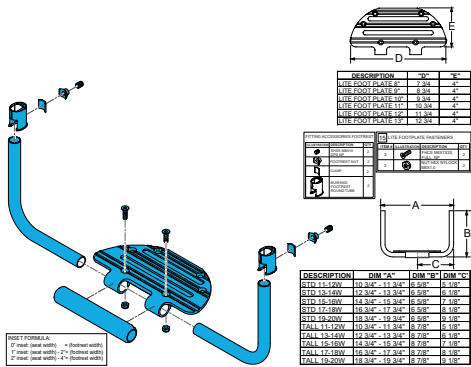
Quickie, Nitrum Ultra-Lite Aluminium Platform Footrest ____" Wide Standard Assembly
