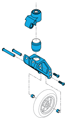
Quickie, Frog Leg Fork and Bearings; With ___ Elastomer
