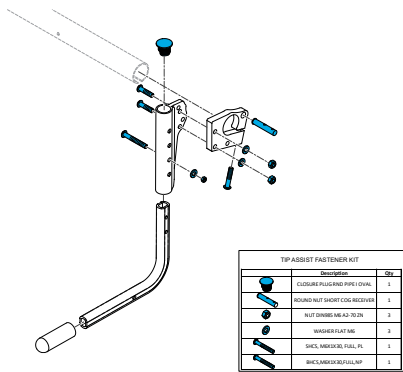
1579-164554 Quickie Rigid Chair, Tip Assist Fastener Kit
