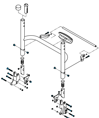
Quickie, Nitrum Back Frame Fasteners Kit; Compatible with Freestyle, Ultra Light Weight Fixed and Height Adjustable Folding Back Frames
