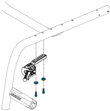
1579-164596 Quickie, Nitrum Direct Mount Compact Wheel Lock Hardware Kit
