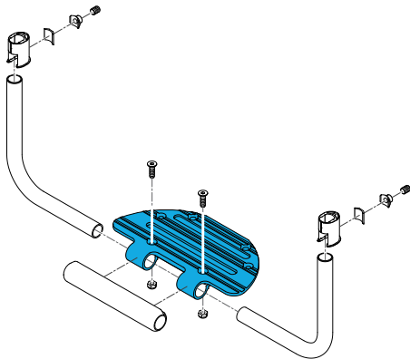
Quickie, Nitrum Ultra-Lite Aluminium Platform ____" Footplate
