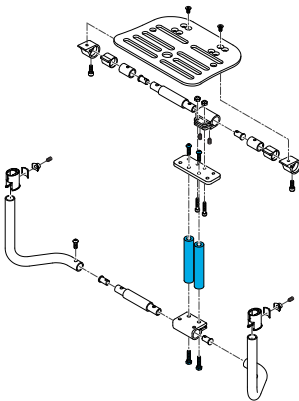
Quickie, Nitrum Platform Footplate Adaptive ___" Spacer Set, Includes Fasteners
