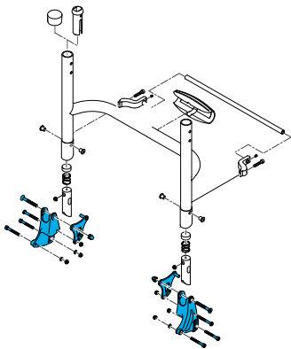
Quickie, Nitrum Ultra Light Weight Back Frame Bracket/Seat Aail Mount Pair
