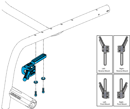
Quickie, Nitrum Compact Wheel Lock, ___ Direct Mount ___ Side
