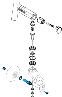
Quickie, Frog Leg Suspension, ___ Elastomer Replacement; For use with ___ kgs
