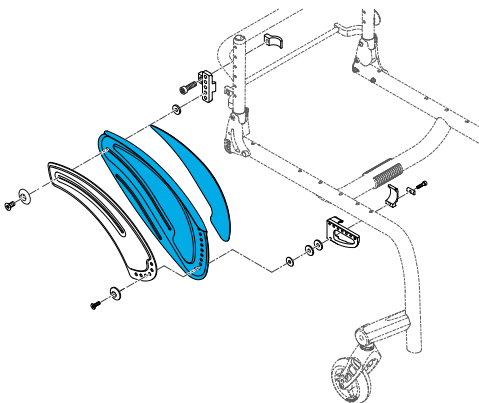
1579-162994 Quickie, Nitrum Carbon Sideguard with Fender Only Right Side
