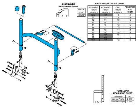
Quickie, Nitrum Ultra Light Weight Fixed Height Back Frame with Narrow Towel Bar for __" Wide Frame
