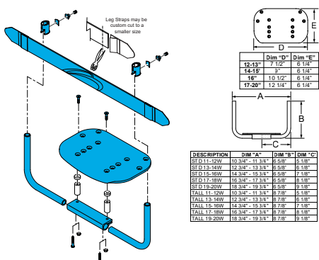
Quickie, Nitrum Composite Footrest Complete Long 12" Wide Assembly
